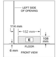
Electrical supply location.
